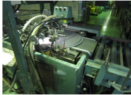
Pre-compounding Machine
